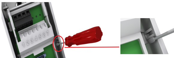
Figure 3 – Removing the Main Unit
