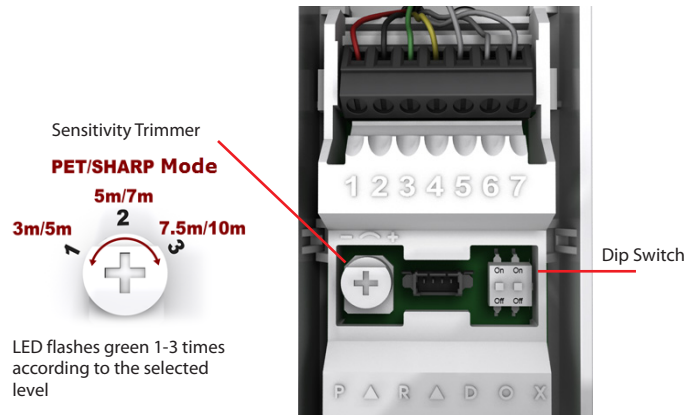
Figure 6 – Detector Settings
